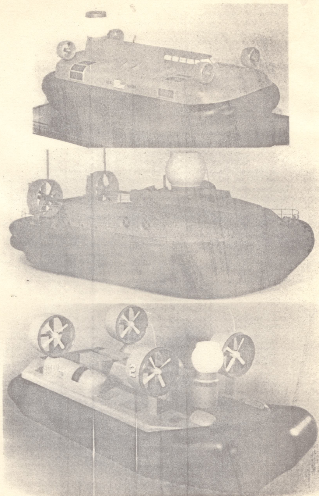
Figure 15. Arctic SEV Models of 150-Ton Aerøjet, 150-Ton Bell, and 500-Ton Boeing Concepts.
