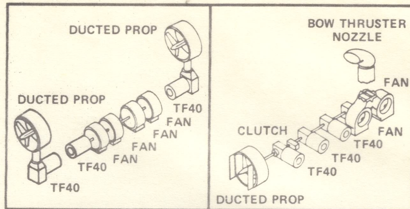
SEPARATED ON JEFF (A) INTEGRATED ON JEFF (B)
