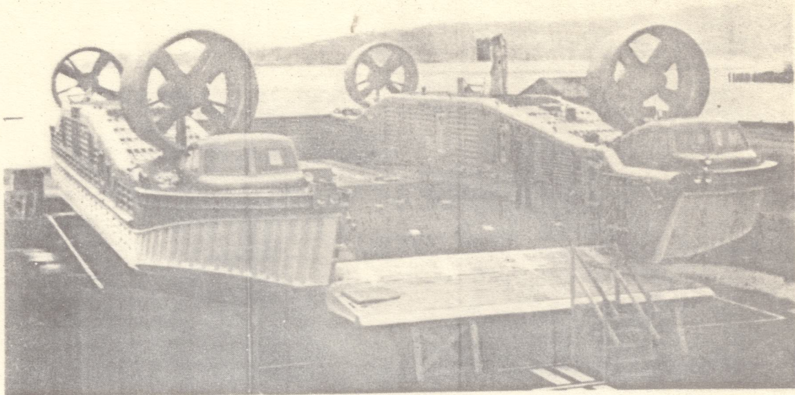
Figure 12. JEFF A Before Skirt Attachment.
