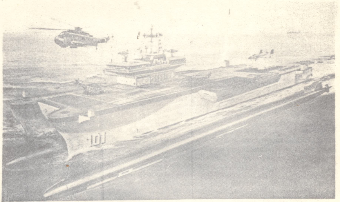
Figure 21. 12000-Ton Air Capable SWATH Ship Concept.
