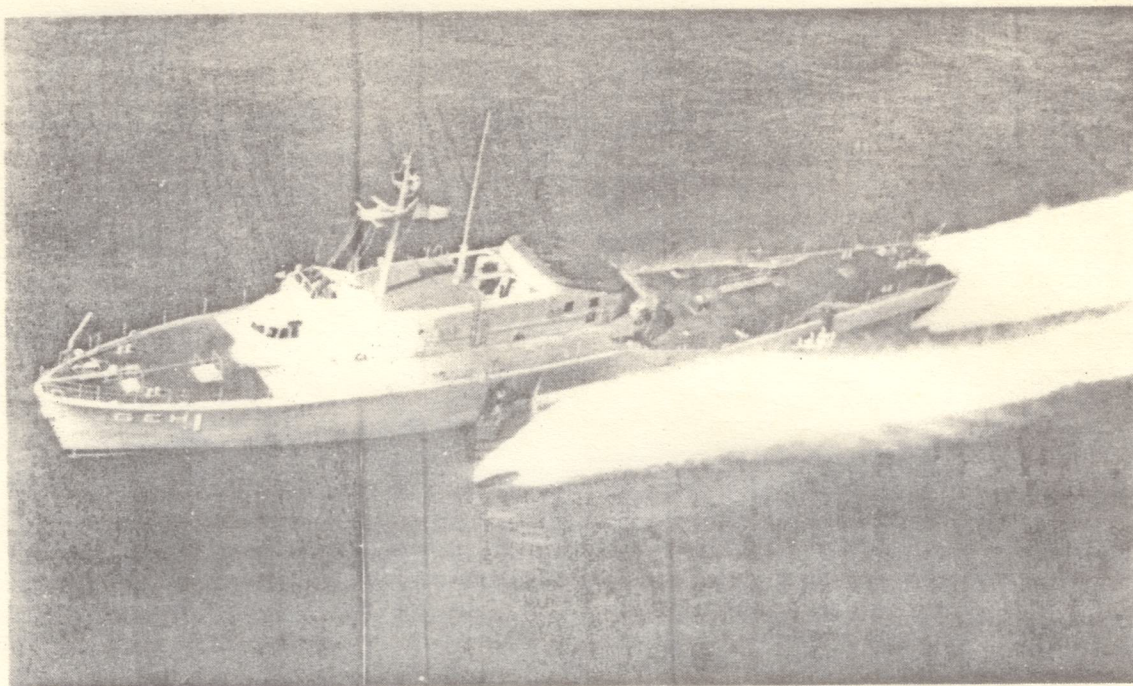
Figure 3. Naval Hydrofoil PLAINVIEW, (AGEH-1).
