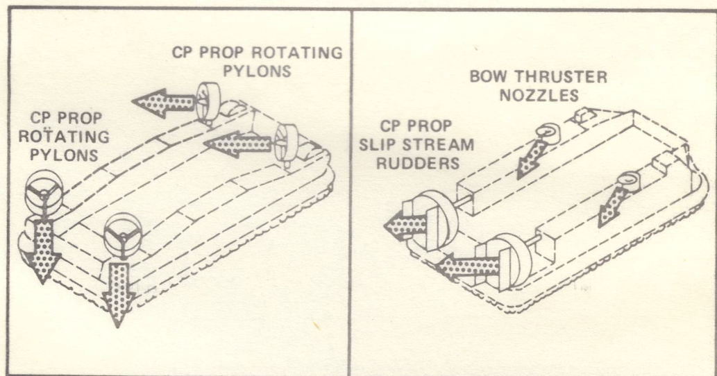
ROTATING PYLONS ON JEFF (A) THRUSTERS/RUDDERS ON JEFF (B)
