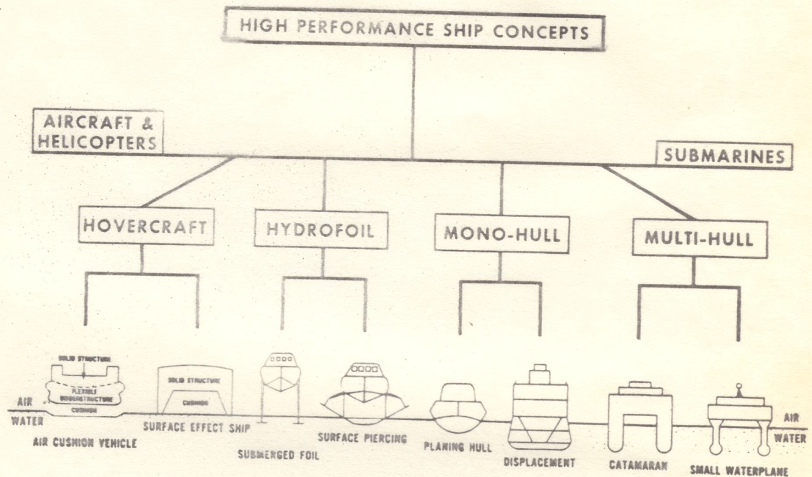
Figure 1. Diagram of Marine Surface Vehicles.
