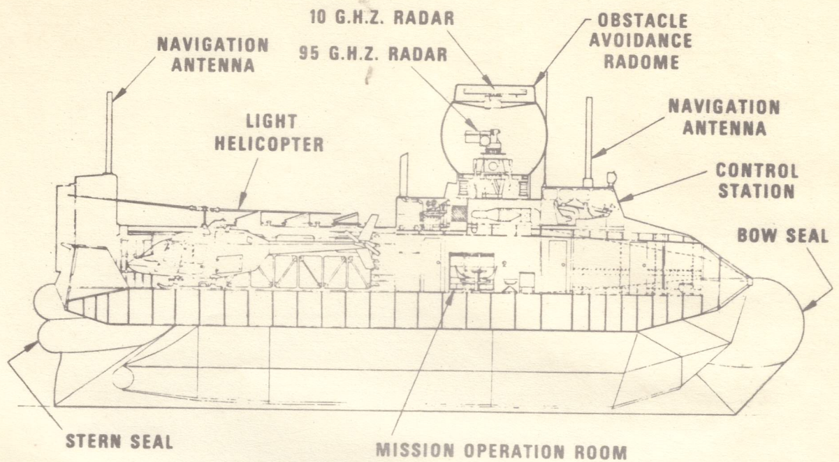
Figure 16. Arrangement of Bell 150-Ton Arctic SEV.
