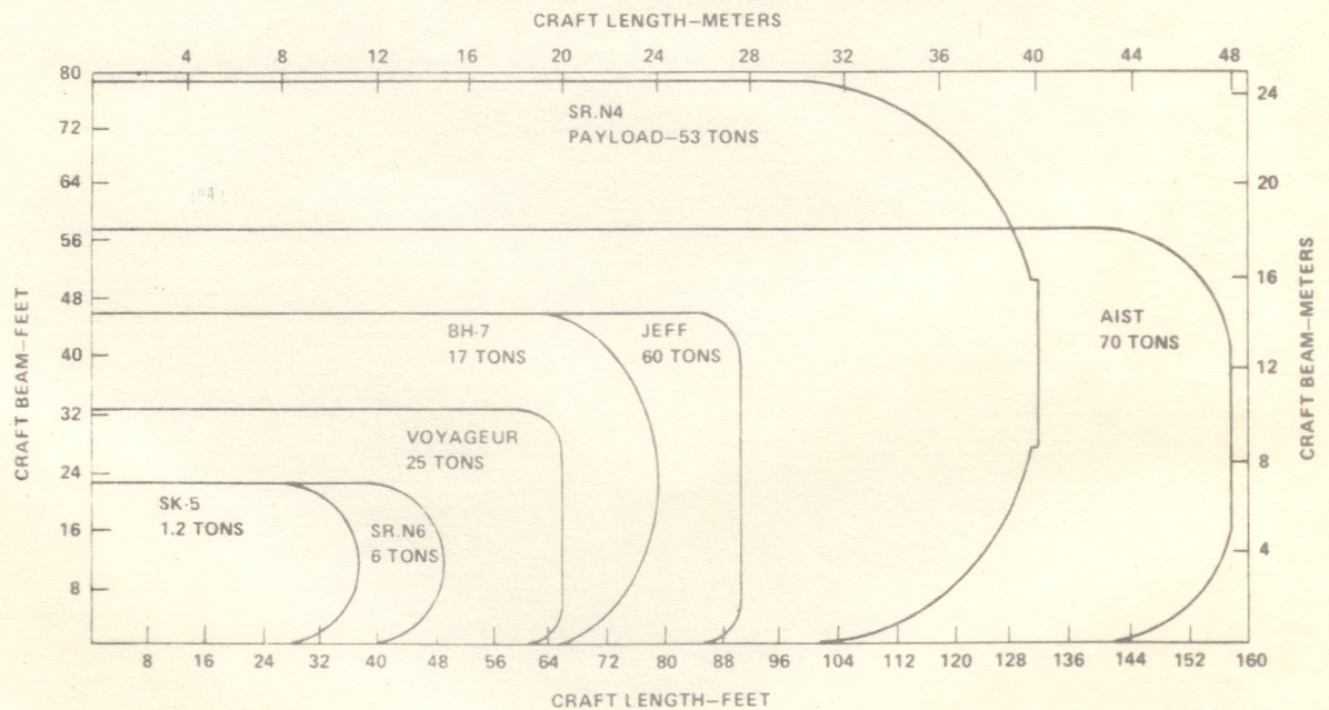
Figure 9. ACV Planform Comparisons.
