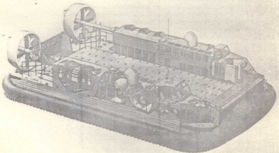
Figure 8. Arrangements of JEFF A and JEFF B Air Cushion Landing Craft.
