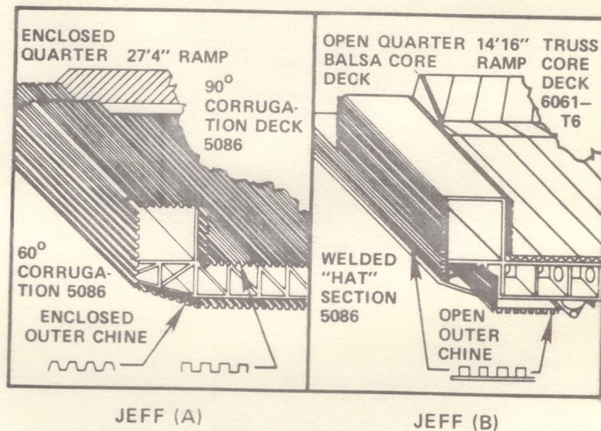
Figure 10b. Comparison of Skirts and Structure.
