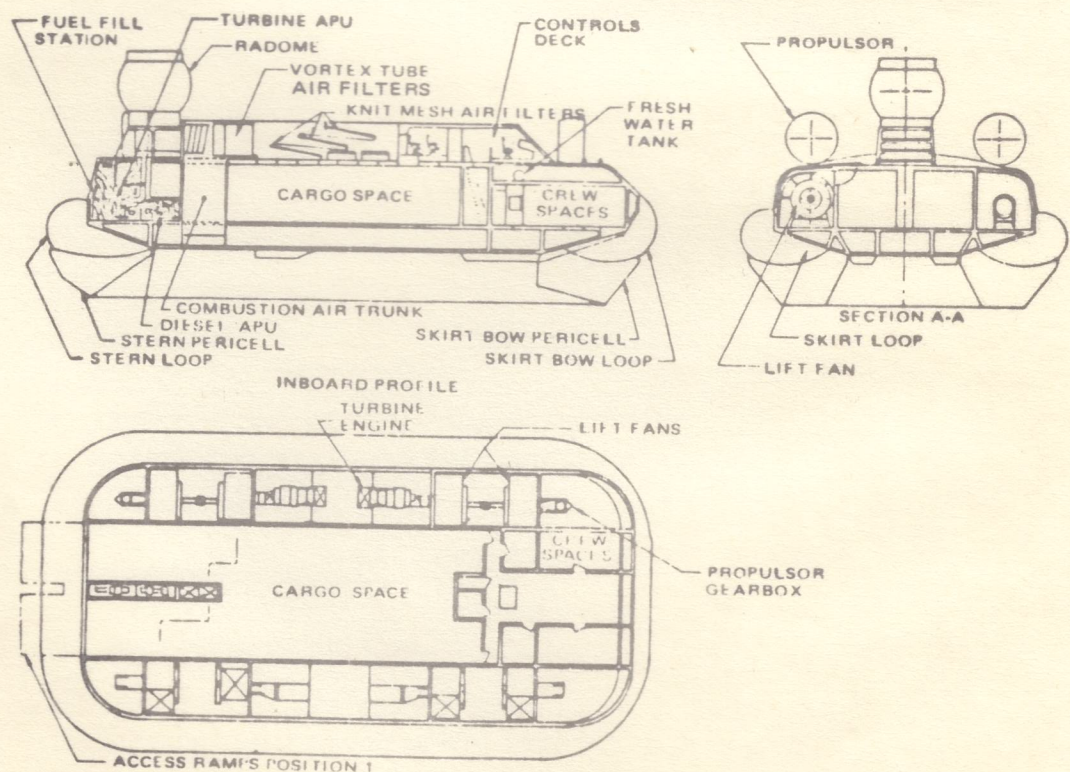
Figure 17. Arrangement of Aerojet 150-Ton Arctic SEV.
